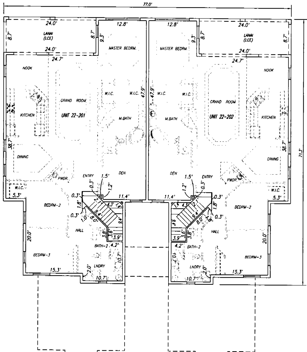
BUILDING '22' SECOND FLOOR (ELEVATIONS IN FEET NGVD29)
