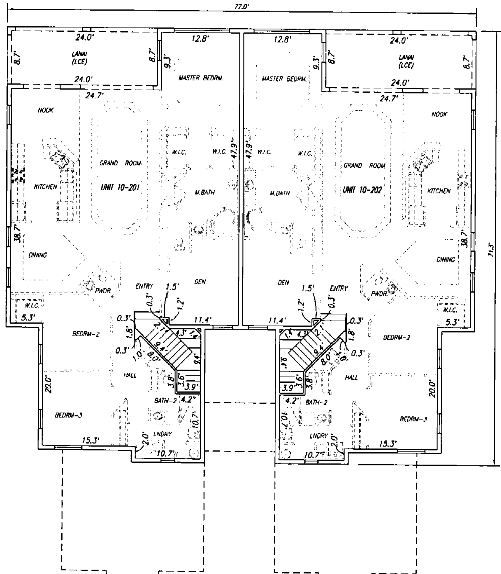
BUILDING "10" SECOND FLOOR (ELEVATIONS IN FEET NGVD29)
