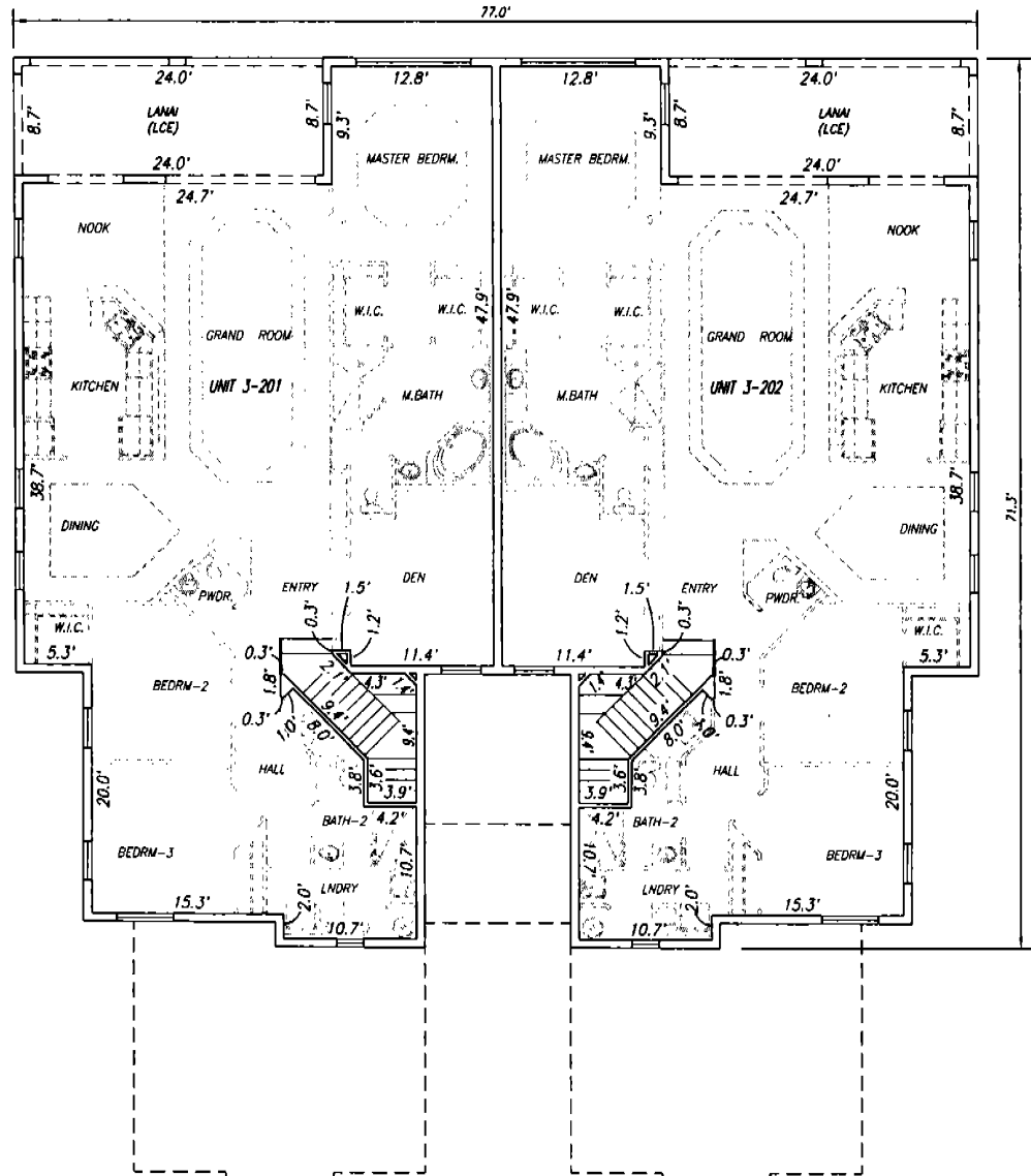
BUILDING "3" SECOND FLOOR (ELEVATIONS IN FEET NGVD29)
