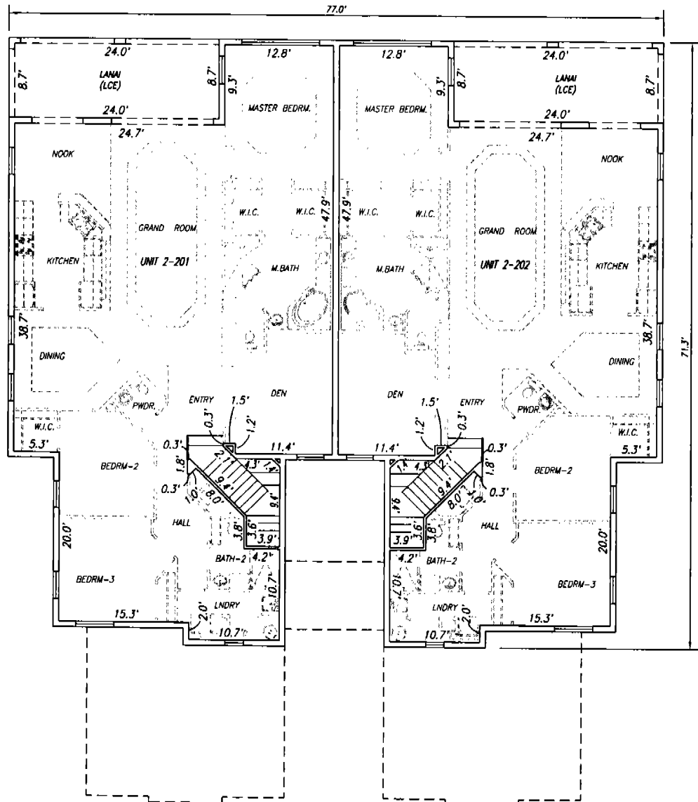
BUILDING '2' SECOND FLOOR (ELEVATIONS IN FEET NGVD29)
