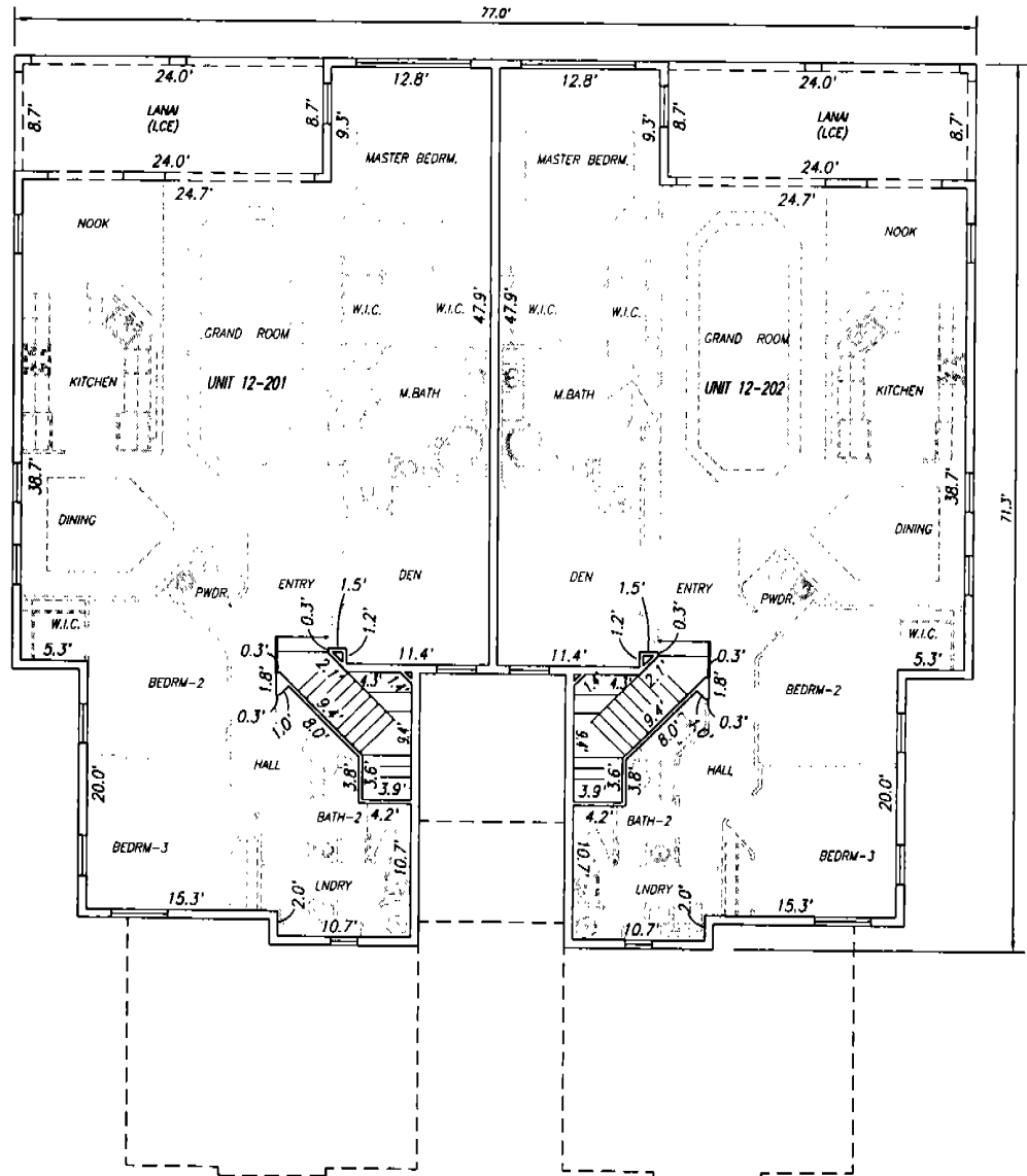
BUILDING '12' SECOND FLOOR (ELEVATIONS IN FEET NGVD29)
