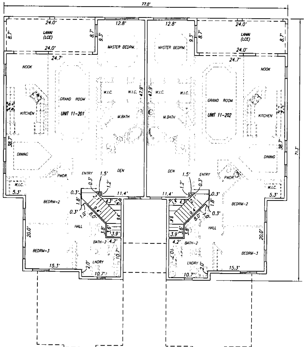
BUILDING "11" SECOND FLOOR (ELEVATIONS IN FEET NGVD29)
