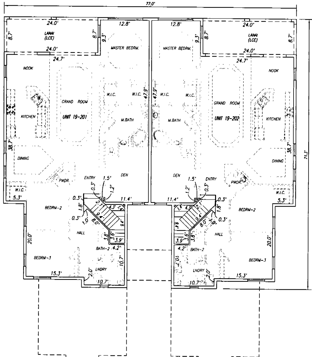
BUILDING '19' SECOND FLOOR (ELEVATIONS IN FEET NGVD29)
