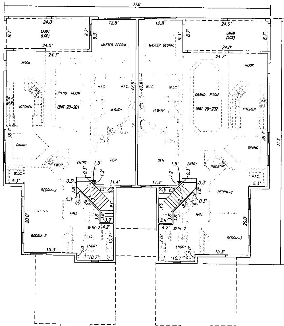
BUILDING '20' SECOND FLOOR (ELEVATIONS IN FEET NGVD29)
