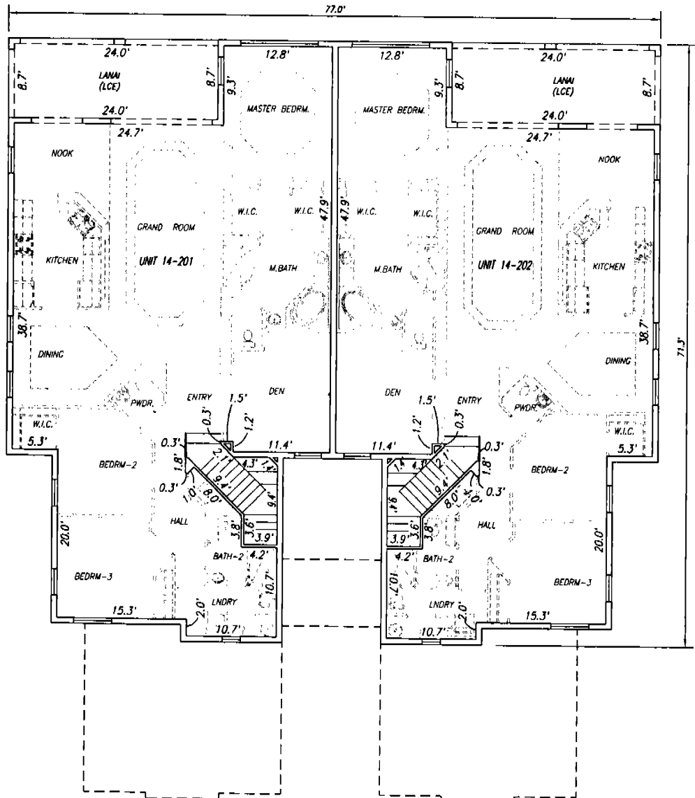
BUILDING '14' SECOND FLOOR (ELEVATIONS IN FEET NGVD29)
