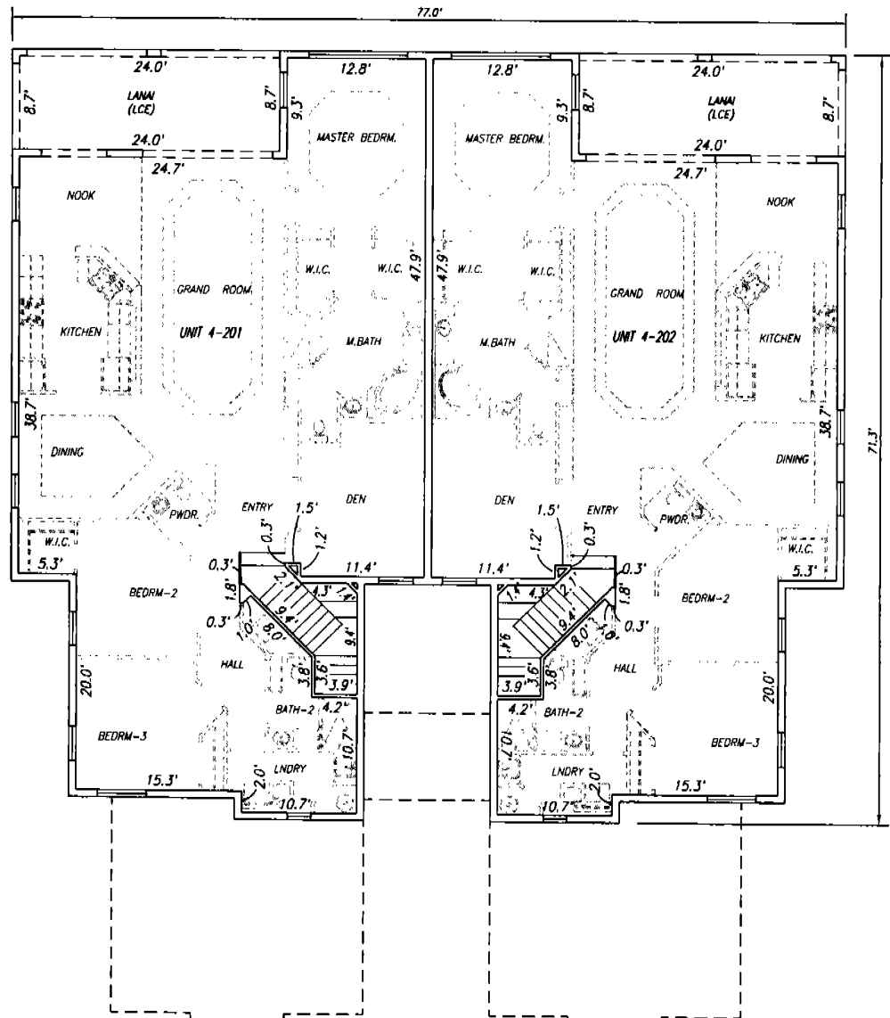
BUILDING '4' SECOND FLOOR (ELEVATIONS IN FEET NGVD29)
