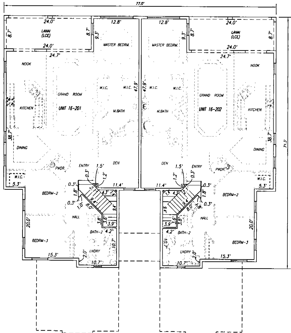
BUILDING '16' SECOND FLOOR (ELEVATIONS IN FEET NGVD29)
