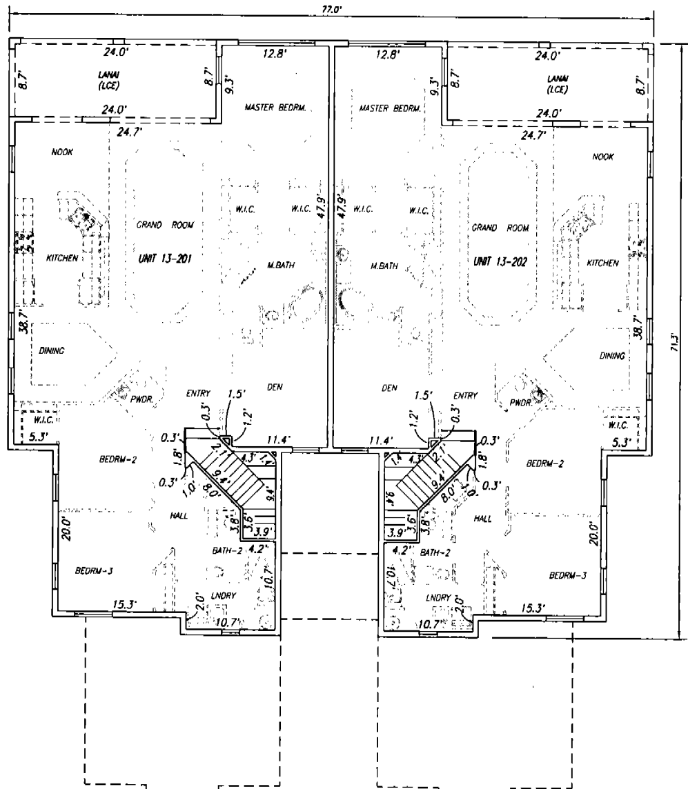
BUILDING '13' SECOND FLOOR (ELEVATIONS IN FEET NGVD29)
