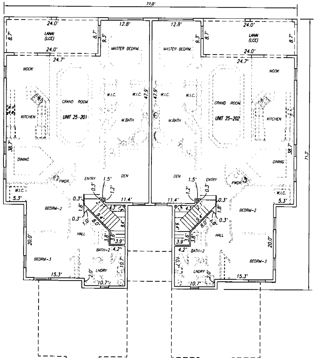
BUILDING '25' SECOND FLOOR (ELEVATIONS IN FEET NGVD29)
