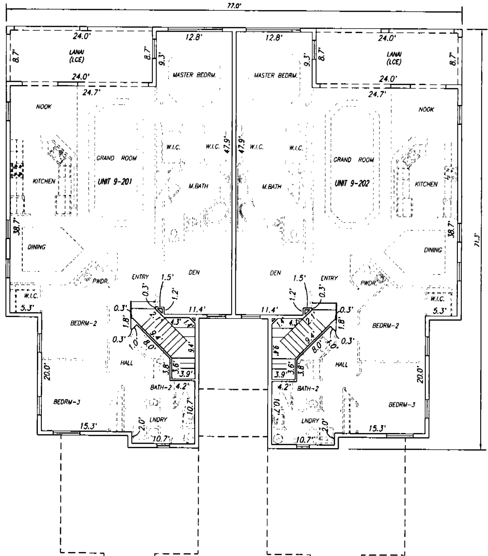
BUILDING '9' SECOND FLOOR (ELEVATIONS IN FEET NGVD29)
