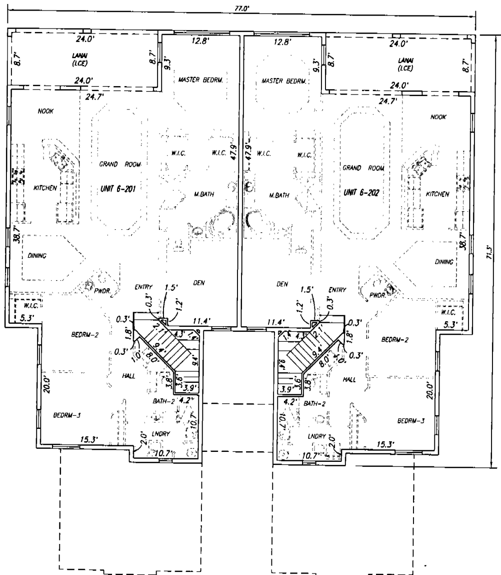
BUILDING '6' SECOND FLOOR (ELEVATIONS IN FEET NGVD29)
